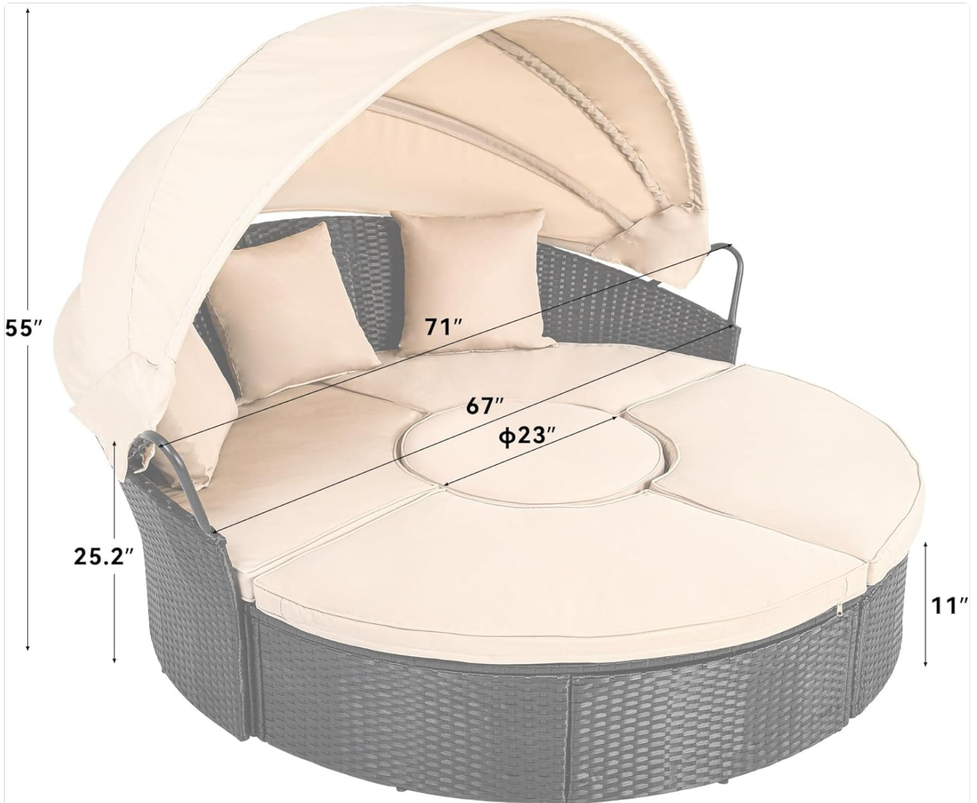
Image 2: Dimensional drawing of the YITAHOME Patio Round Daybed.
