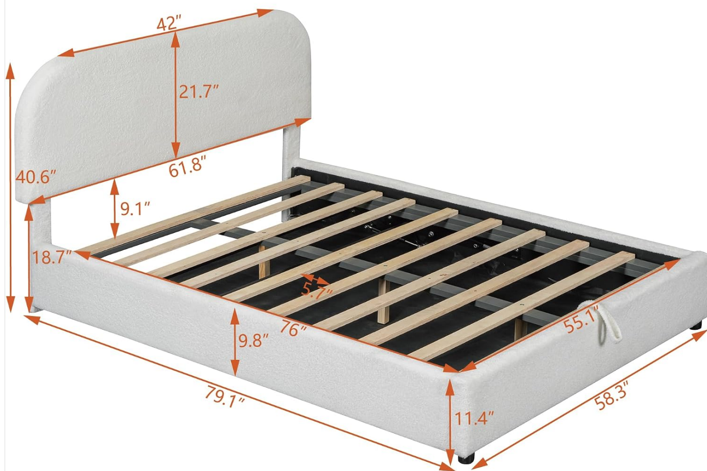
Image: The bed with the hydraulic storage system in the open position, showing the storage space.
