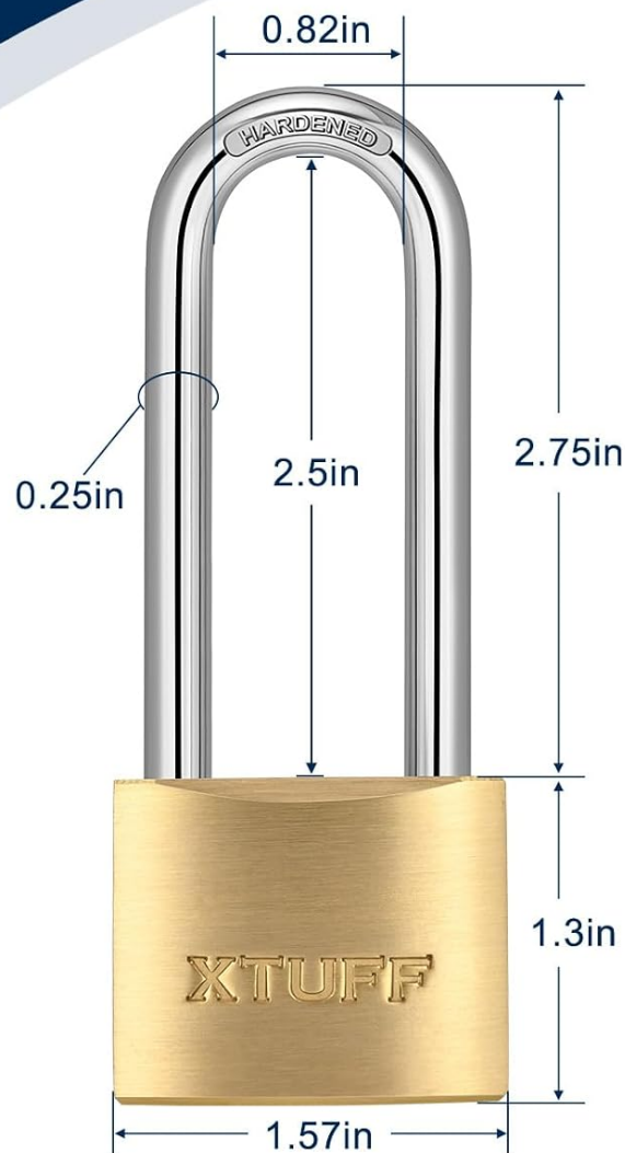
Image: Detailed product dimension diagram for the XTUFF padlock.
