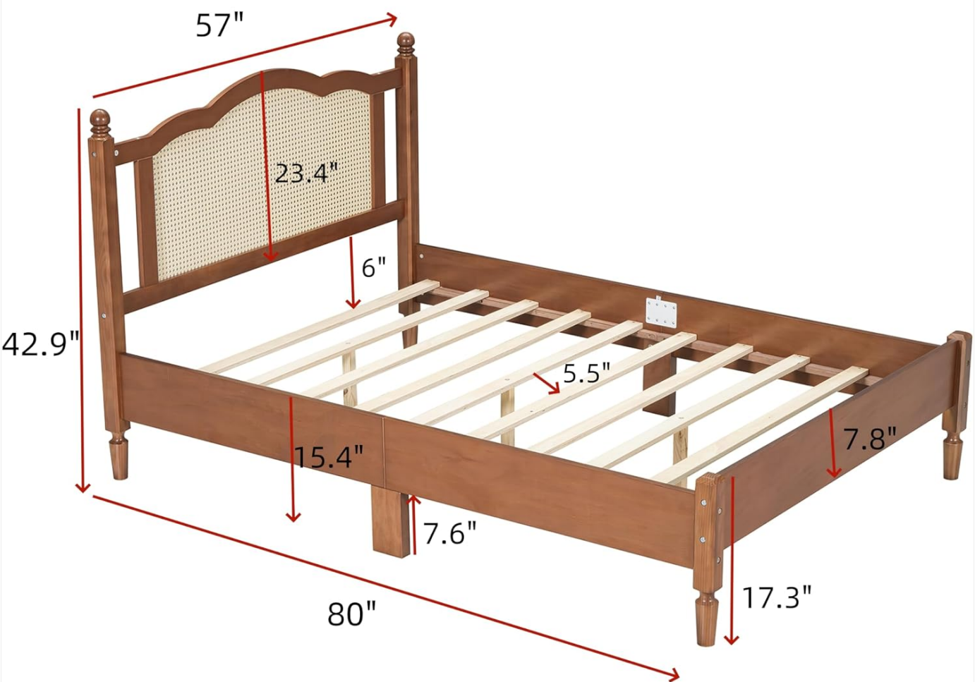
Image: Detailed dimensions of the bed frame, including length, width, and height measurements for various components.
