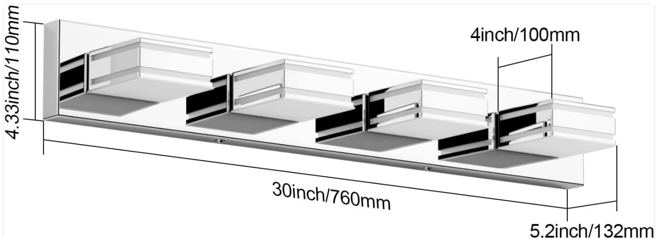
Figure 2: Product dimensions, showing the length of 30 inches (760mm) and other measurements for installation planning.
