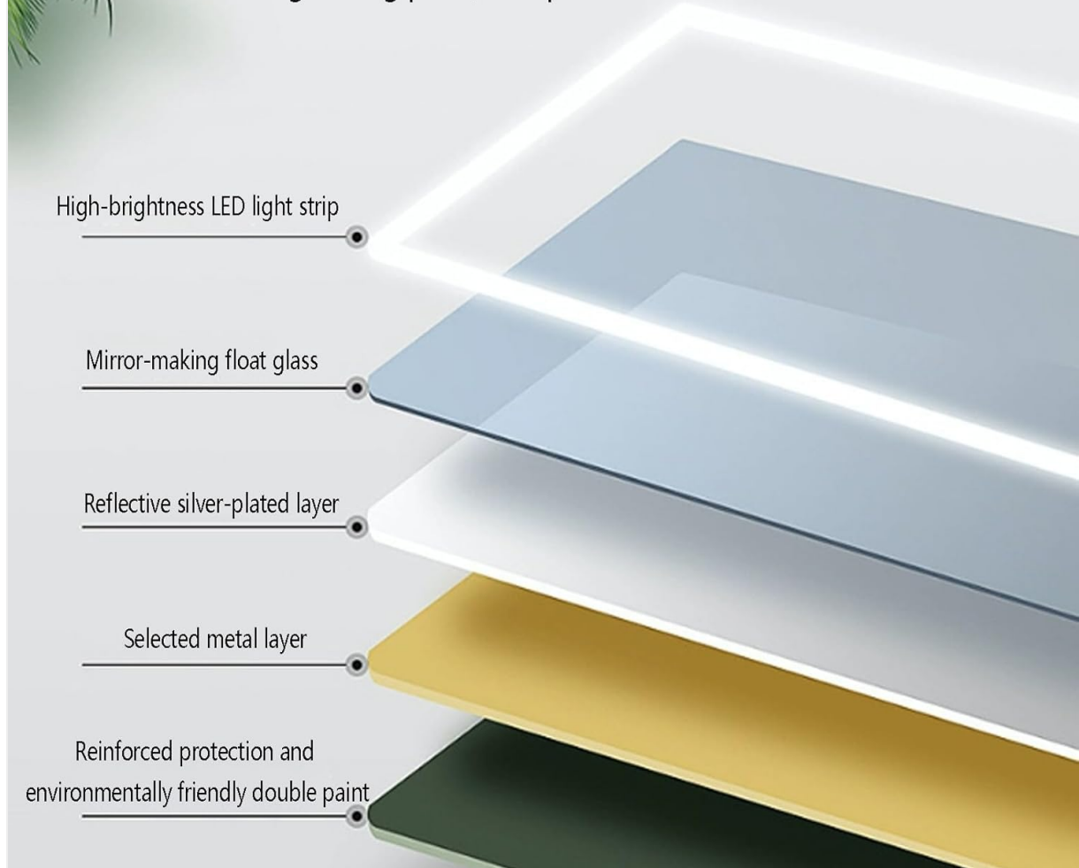
Image 4.2: Cross-section view of the mirror's construction, highlighting the high-brightness LED light strip, float glass, reflective silver-plated layer, selected metal layer, and reinforced protection.
