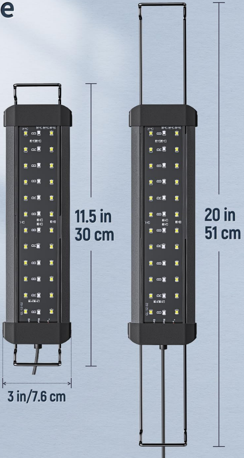
Image: The Pawfly LED Light demonstrating its extendable design, suitable for 12 to 18-inch tanks. Specifications include LUX: 2500, PAR: 55, CRI: 90, Power: 9 W. Dimensions shown are 11.5 in (30 cm) extending to 20 in (51 cm) with a width of 3 in (7.6 cm).
