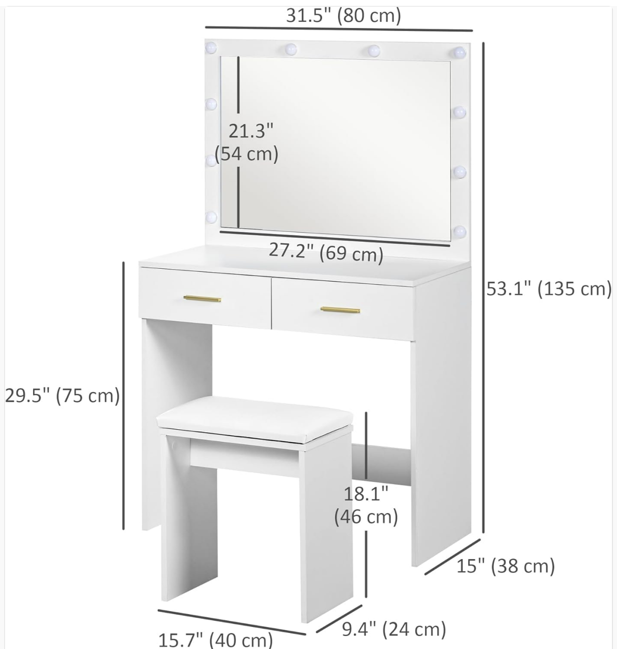
Image 4.1: Dimensions of the vanity desk and stool for planning placement.
