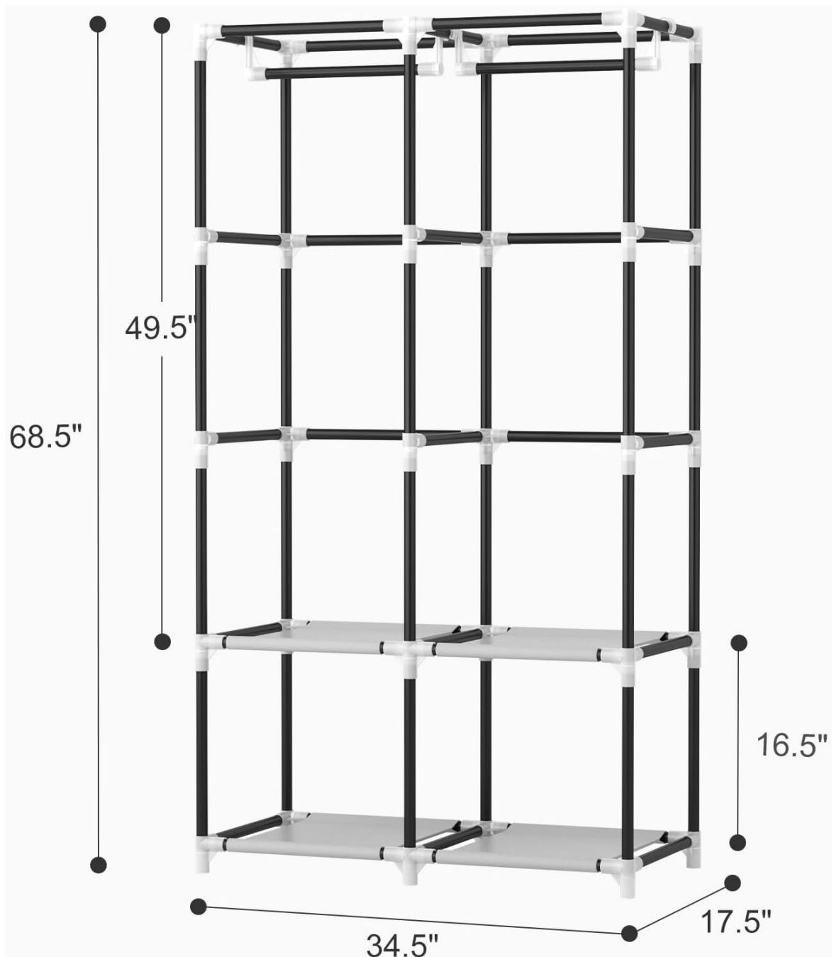
Figure 2: Overall dimensions of the assembled closet.
