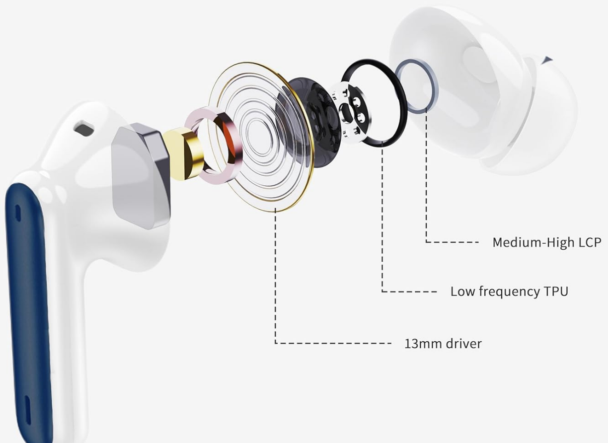
Figure 5: Internal structure highlighting the 13mm high-efficiency speaker for immersive audio.
