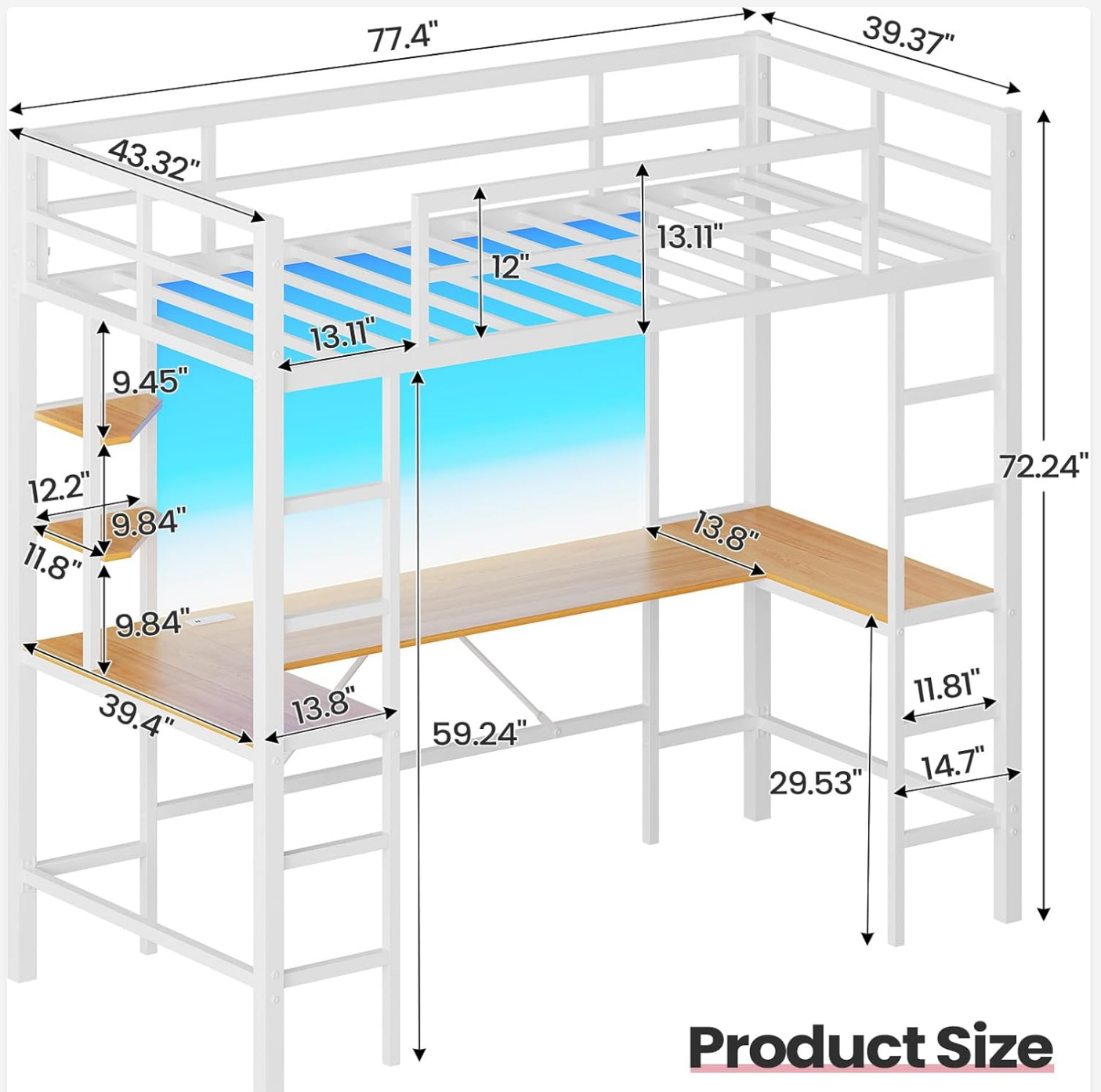
Figure 4.1: Product Dimensions and Structure. This diagram illustrates the overall size and key structural elements of the loft bed.
