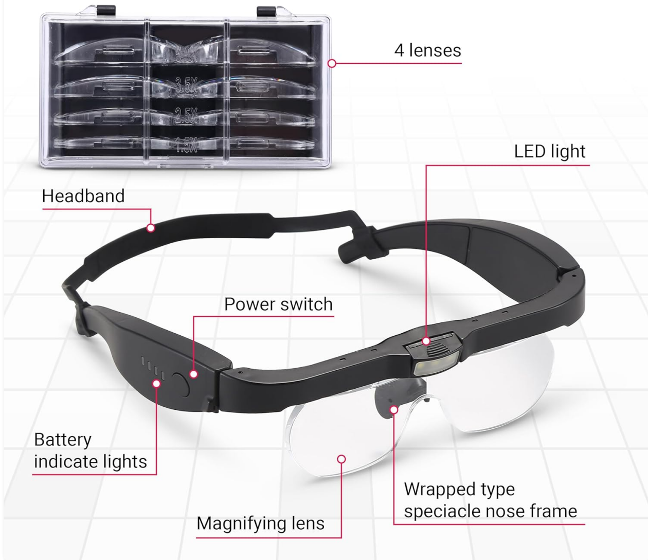
Figure 2: Labeled diagram of the magnifying glasses components, including lenses, LED light, power switch, battery indicator, and nose frame.
