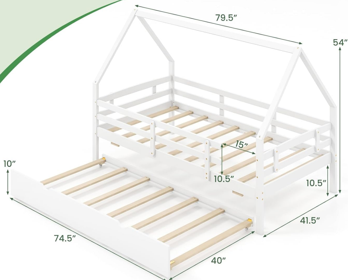
Figure 2: Key dimensions and specifications for assembly planning.
