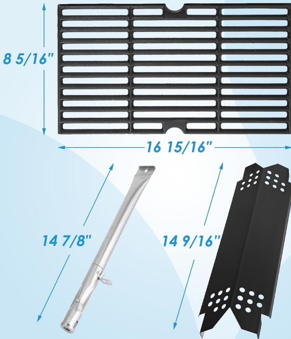
Image: A detailed diagram illustrating the precise dimensions of the cooking grates, burners, and heat plates included in the kit.
