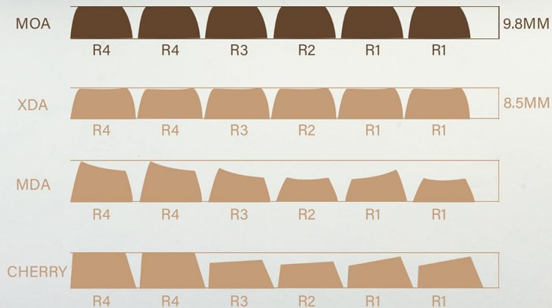
Figure 3.1: Comparison of MOA keycap profile with other common profiles, illustrating its unique ergonomic shape and height.
