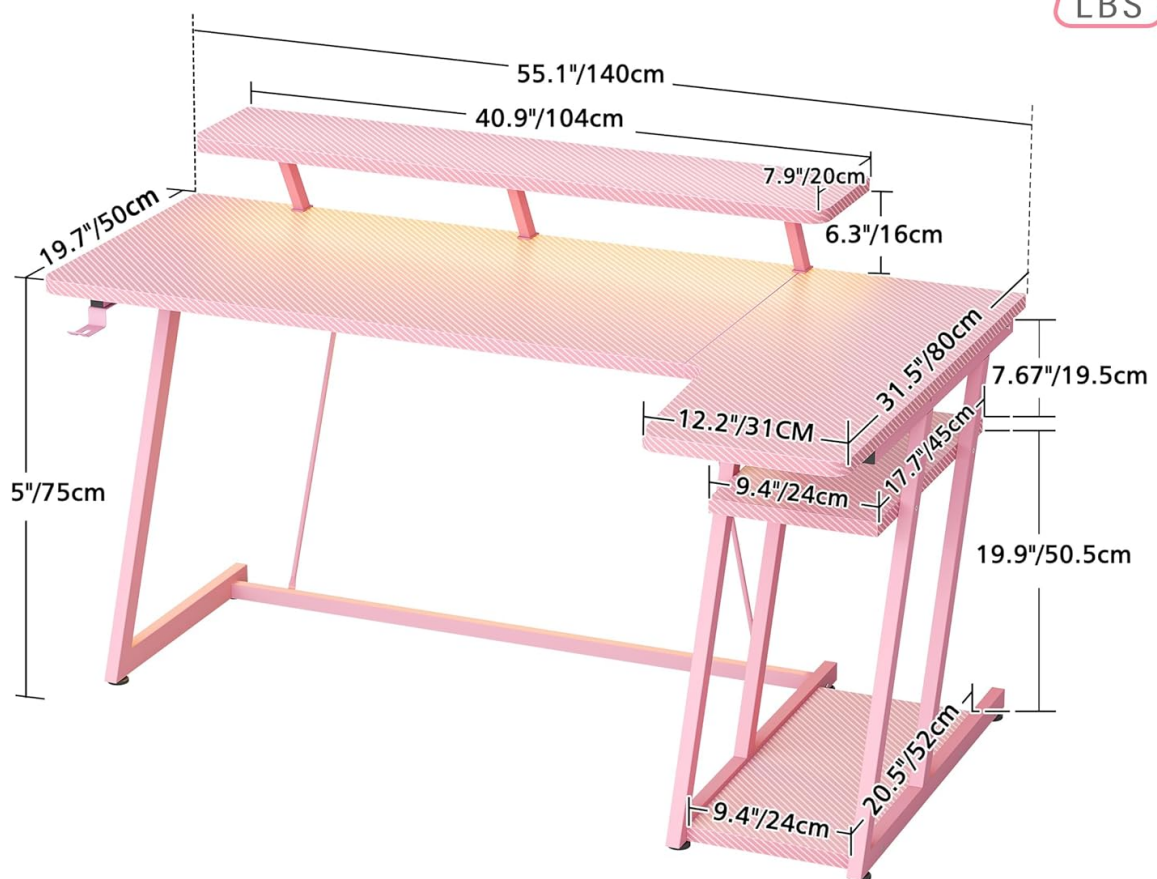
Image: Detailed diagram illustrating the dimensions of the HOMIDEC Gaming Desk, including the main desktop, monitor stand, and storage shelves.
