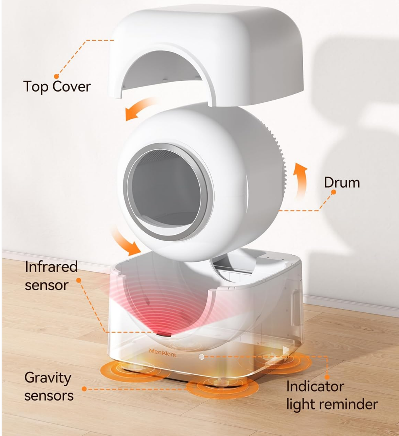
Figure 2: Components and sensor locations for safe operation.
