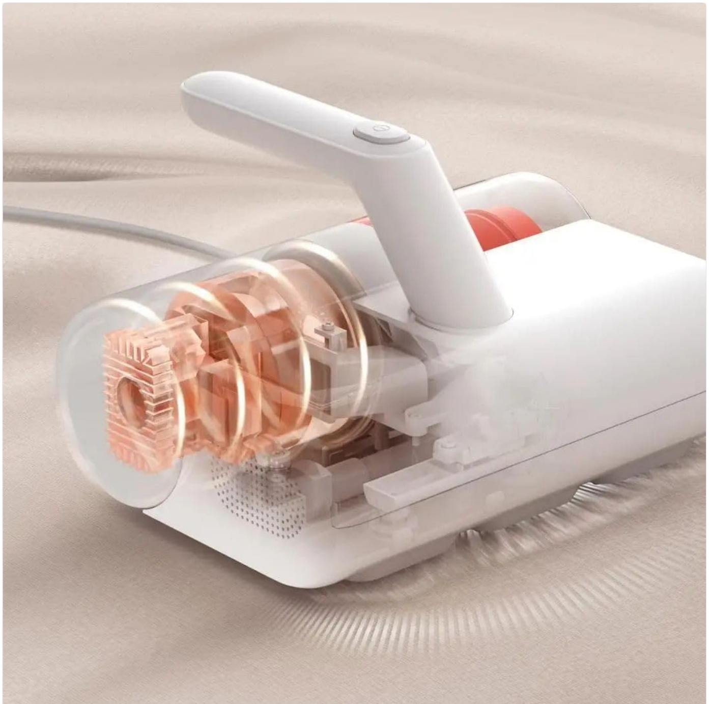
Figure 4: Transparent view illustrating the internal motor and fan assembly responsible for powerful suction.
