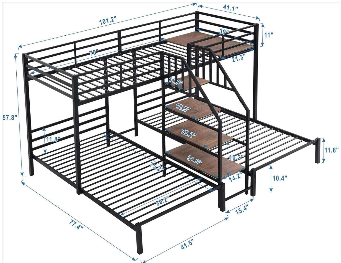
Image: Detailed dimensions of the bunk bed frame, useful for planning placement and assembly.
