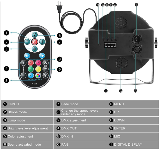
Figure 4.1: Back Panel and Remote Control
