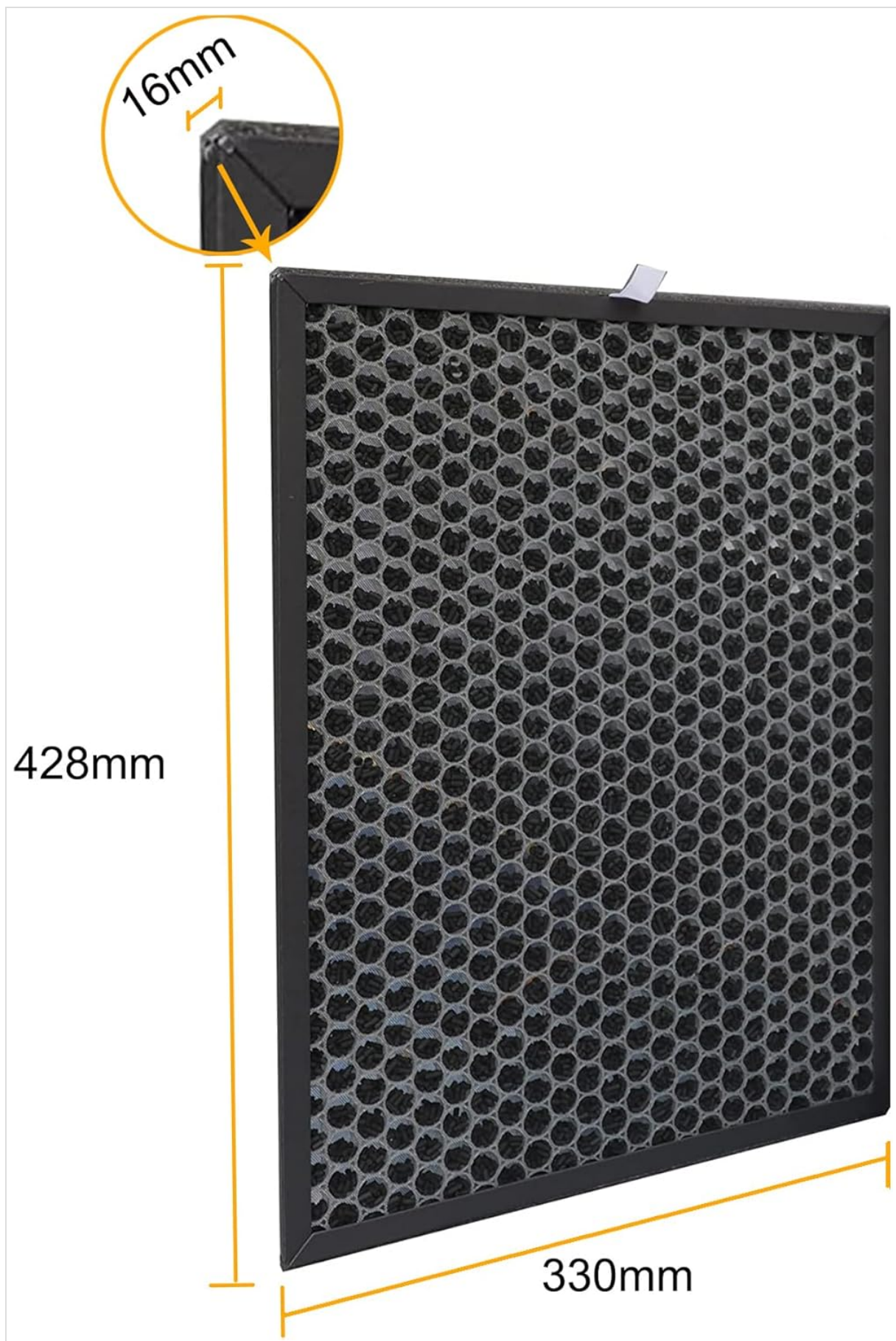
Image 5: Detailed dimensions of the Activated Carbon filter (428mm x 330mm x 16mm).
