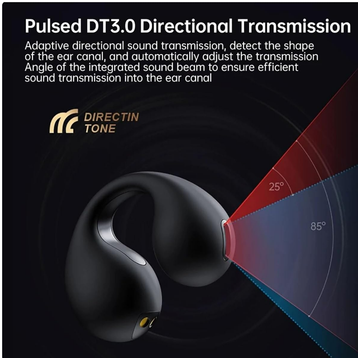
Image: A diagram illustrating the Pulsed DT3.0 Directional Transmission technology, showing how sound is precisely directed into the ear canal.
