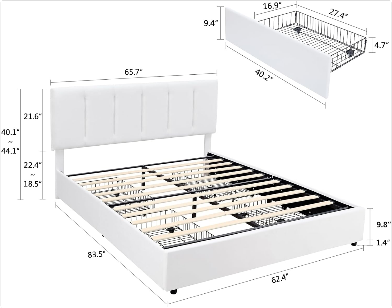
Image: A technical diagram illustrating the precise dimensions of the VECELO Queen Size Bed Frame, including overall length, width, headboard height range, and storage drawer dimensions.
