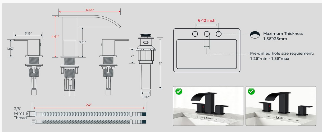
Figure 4.1: Faucet dimensions and sink compatibility requirements for installation.
