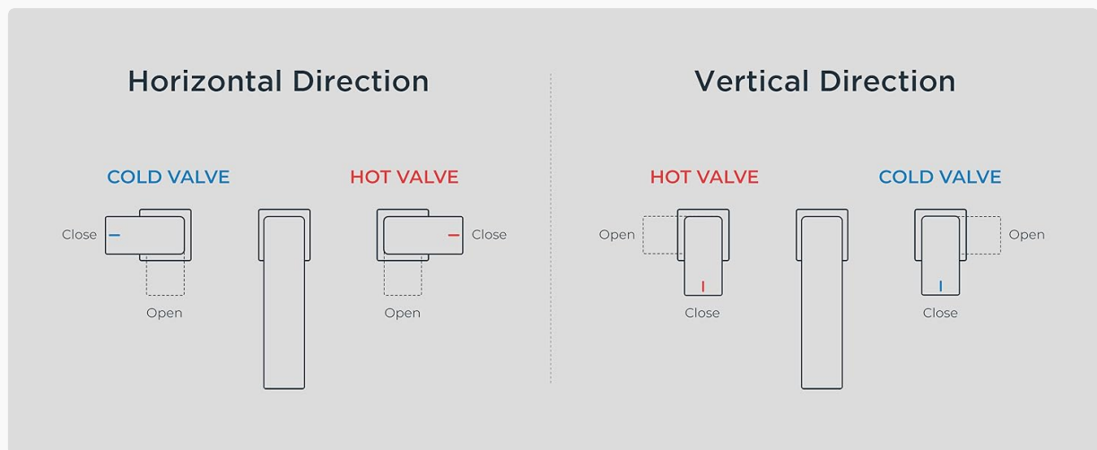
Figure 5.1: Illustration of handle operation for controlling hot and cold water in both horizontal and vertical directions.
