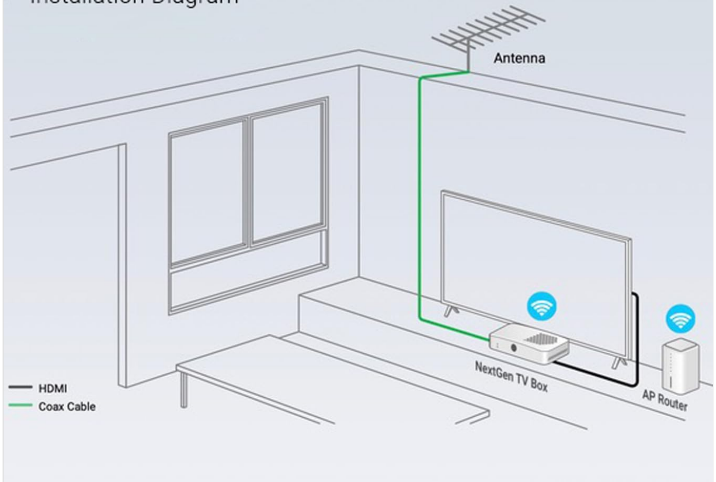
Image: An installation diagram illustrating how to connect the Zinwell NextGen TV Box. It shows an antenna connected to the box via a coaxial cable, and the box connected to a TV via an HDMI cable. An optional Wi-Fi router connection is also depicted.
