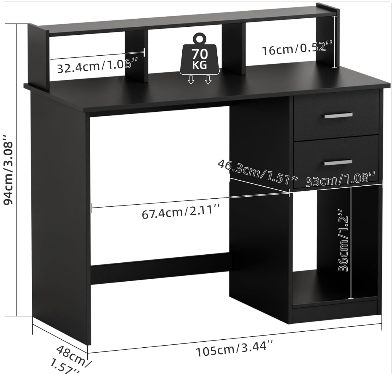
Image 3.1: Overview of desk dimensions and main components. This image illustrates the overall size of the desk (105cm width, 48cm depth, 94cm height) and highlights key sections like the desktop, upper shelves, drawers, and lower open compartment. It also indicates a maximum load capacity of 70 kg for the desktop.
