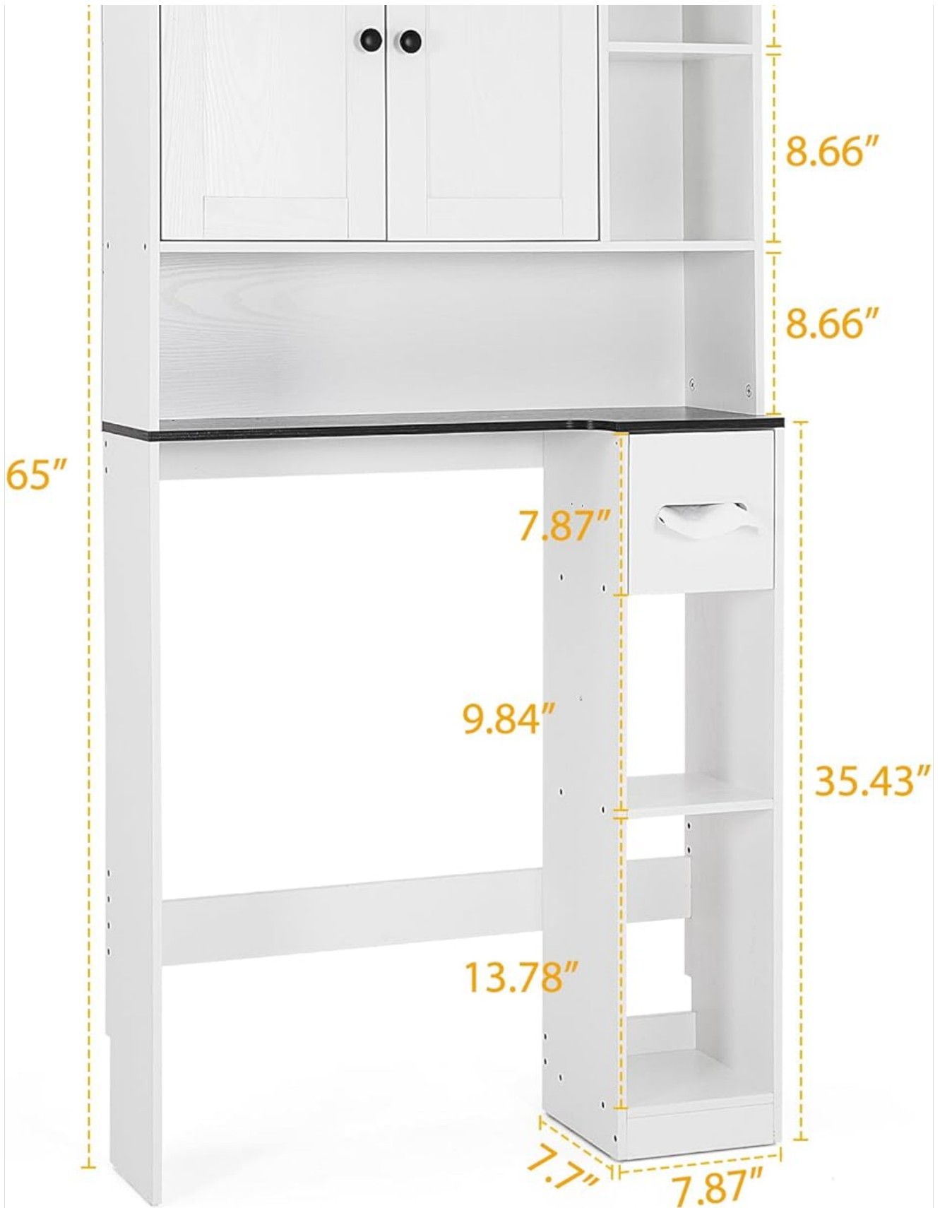
Image 7.1: Detailed dimensions of the cabinet, including height, width, and depth, to assist with space planning.
