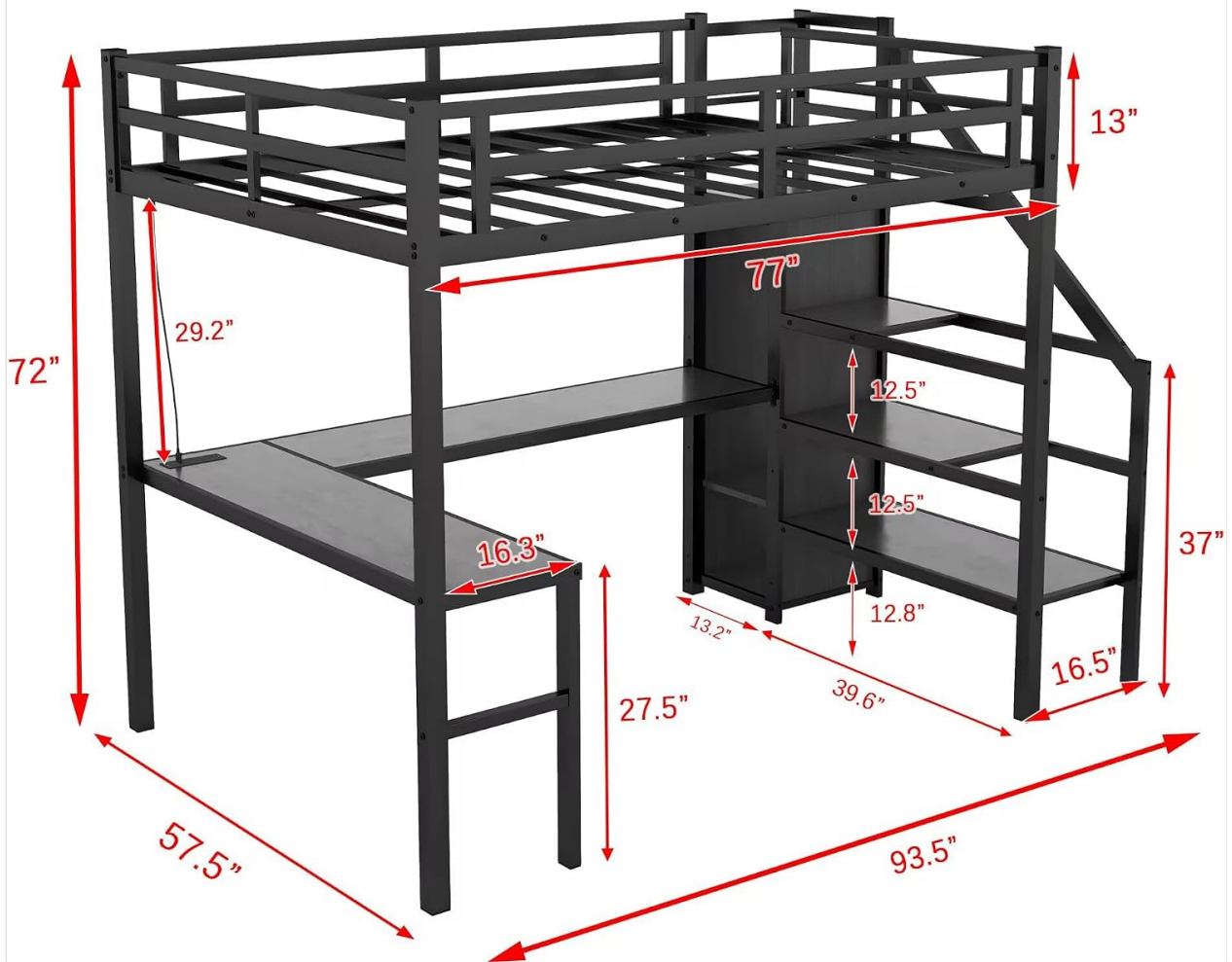
Figure 3.1: Overall dimensions of the loft bed, including bed frame, desk, and staircase. Dimensions are 93.5 inches (L) x 57.5 inches (W) x 72 inches (H).
