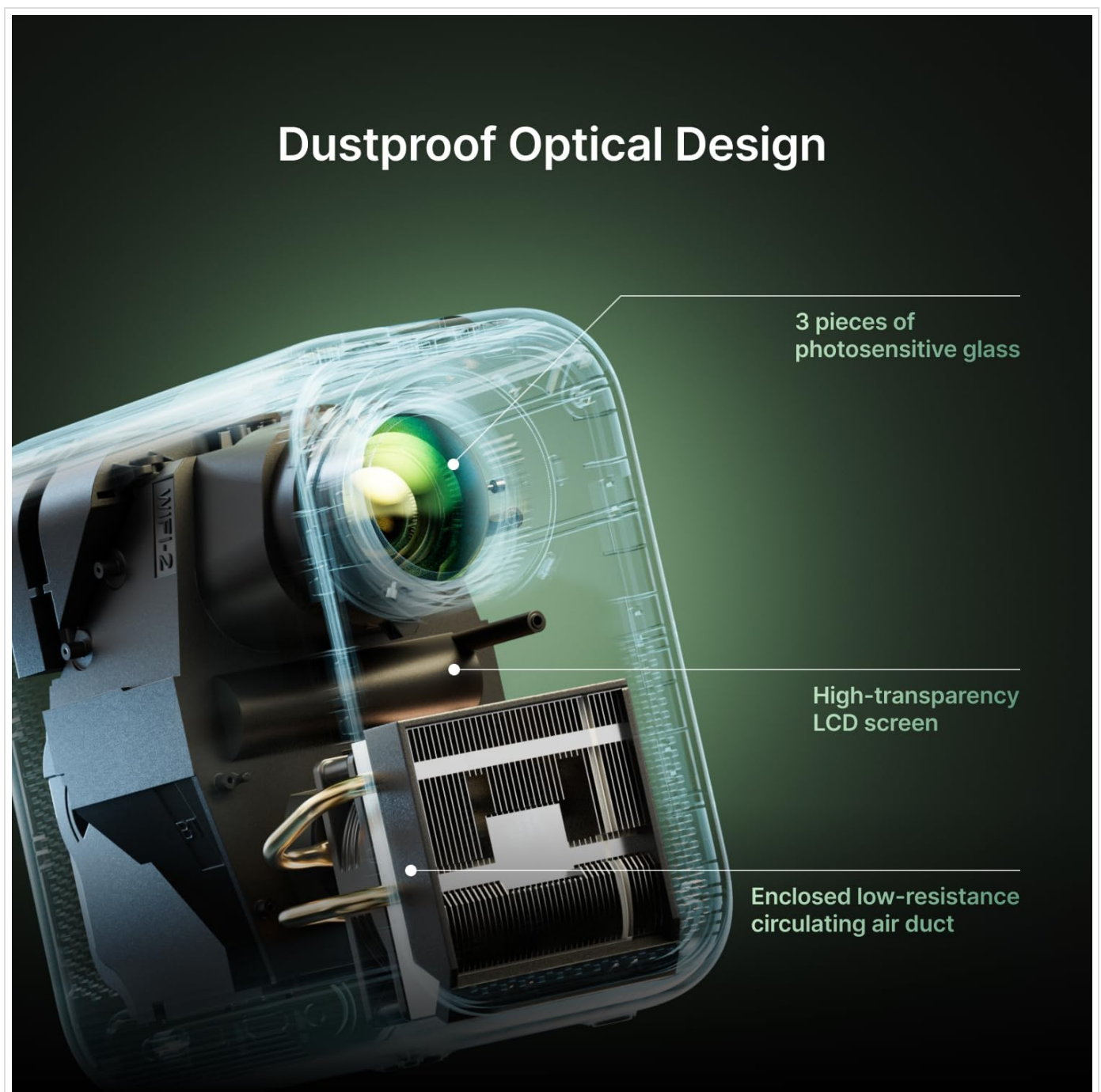
Image: An internal diagram illustrating the projector's dustproof optical design, featuring multiple glass elements and an enclosed air duct for protection.
