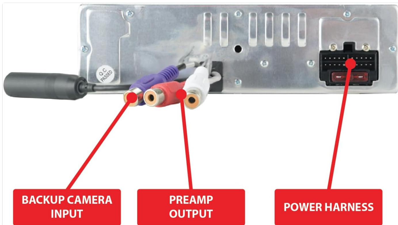
Figure 2: Rear connections of the XDVD179BT, highlighting the backup camera input, preamp output, and power harness port.
