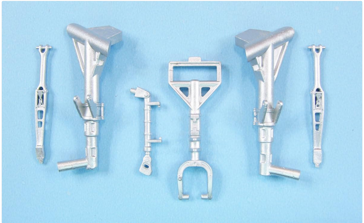
Figure 2: Individual metal landing gear components. These parts replace the plastic equivalents in the Meng 1:48 J-20 kit.
