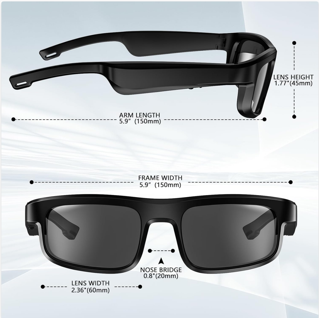
Image 5.1: Diagram showing the dimensions of the smart glasses, including lens height (1.77"/45mm), arm length (5.9"/150mm), frame width (5.9"/150mm), lens width (2.36"/60mm), and nose bridge (0.8"/20mm).
