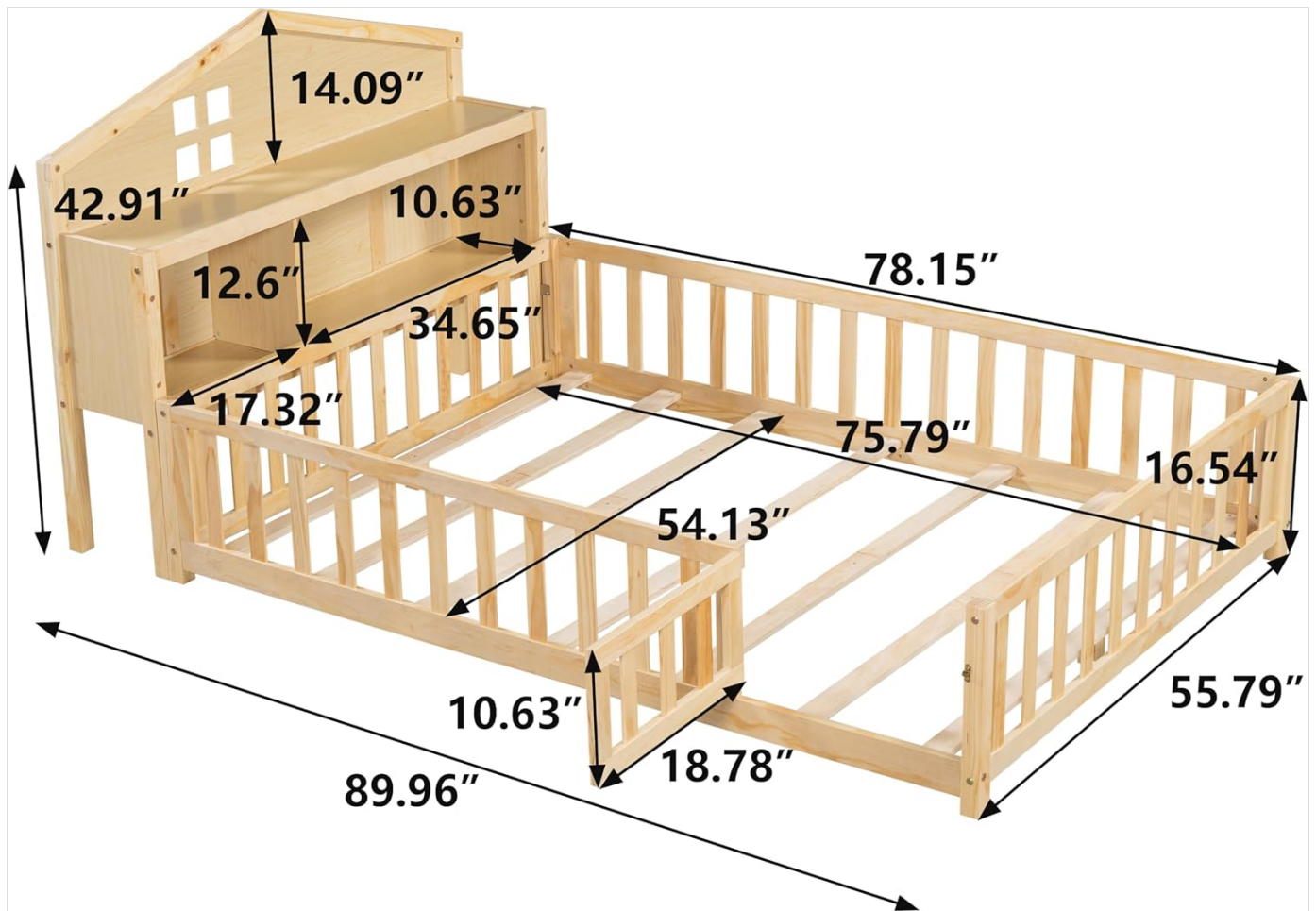
Figure 1: Overall dimensions of the Bellemave Full Size Montessori Floor Bed.
