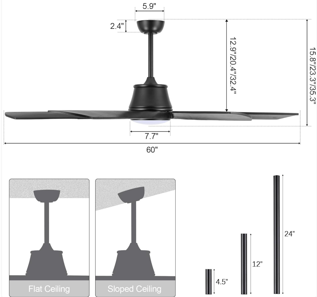
Figure 2: Product dimensions and compatibility with flat and sloped ceilings.
