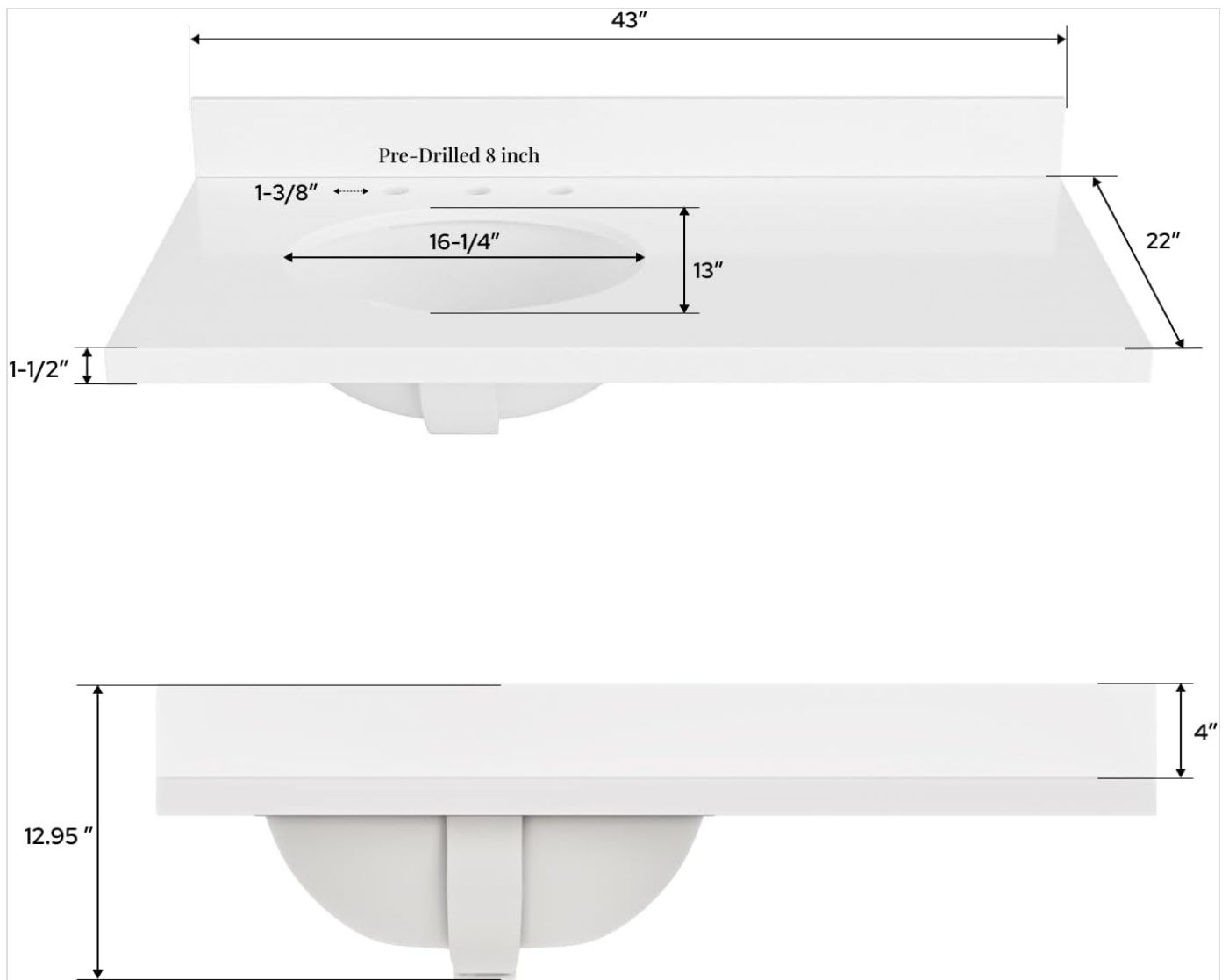
Image: Detailed dimensions of the ARIEL 43 inch vanity top, showing length, width, sink dimensions, and backsplash height.
