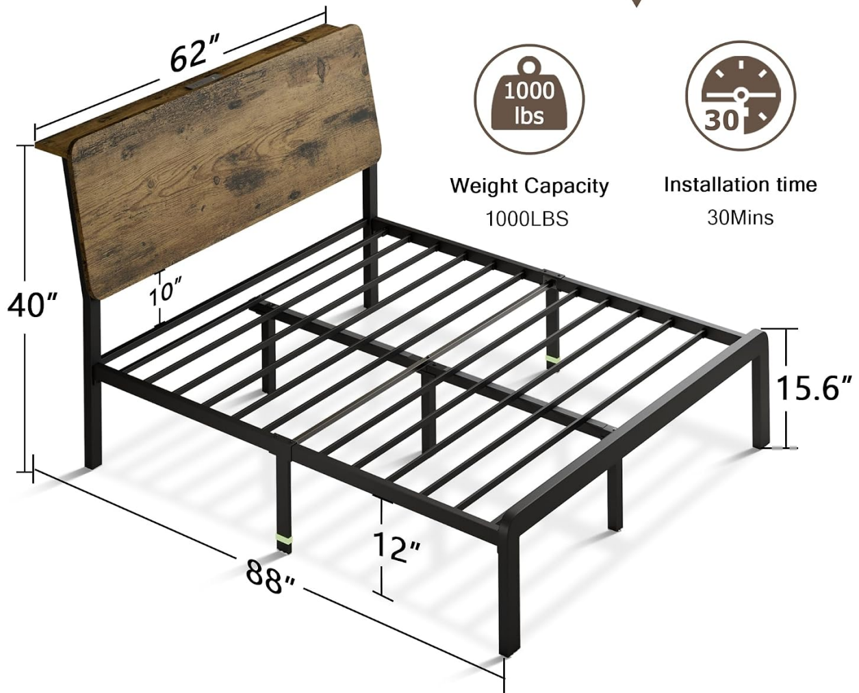
Figure 1: Einhorn Queen Bed Frame dimensions and key specifications.
