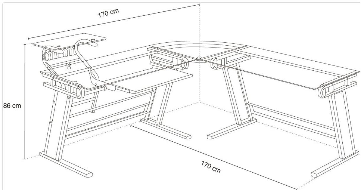
Figure 2: Dimensional diagram illustrating the overall size and L-shape configuration of the desk, crucial for planning your workspace. Dimensions are approximately 170 cm (Length) x 170 cm (Width) x 86 cm (Height).
