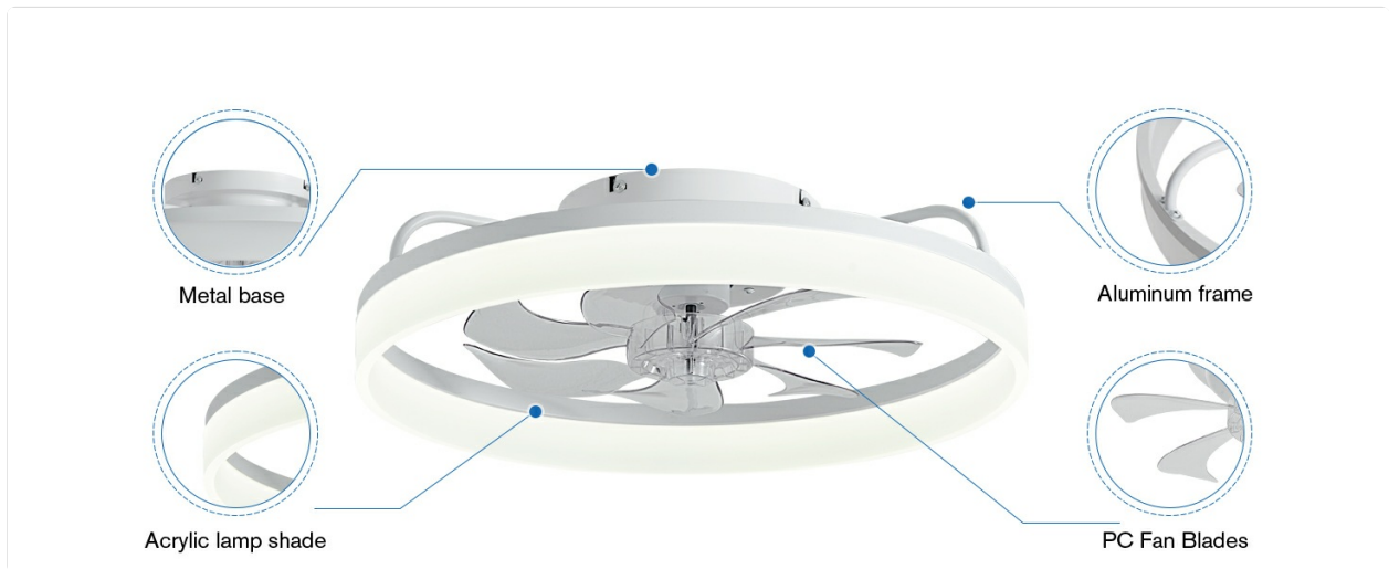
Figure 4.2: Key components of the AQUBT Ceiling Fan, highlighting the metal base, aluminum frame, acrylic lampshade, and PC fan blades.
