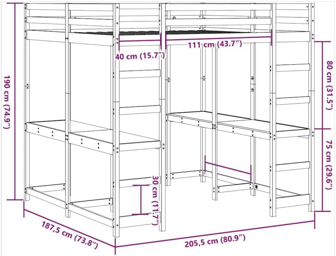
Image 4.1: Detailed dimensions diagram of the bunk bed structure.
