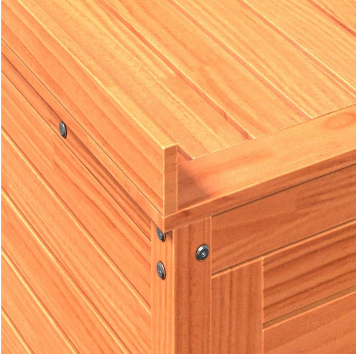
Figure 4.1: A detailed view of a corner joint, highlighting the secure screw fasteners used in the assembly of the solid pine wood panels.
