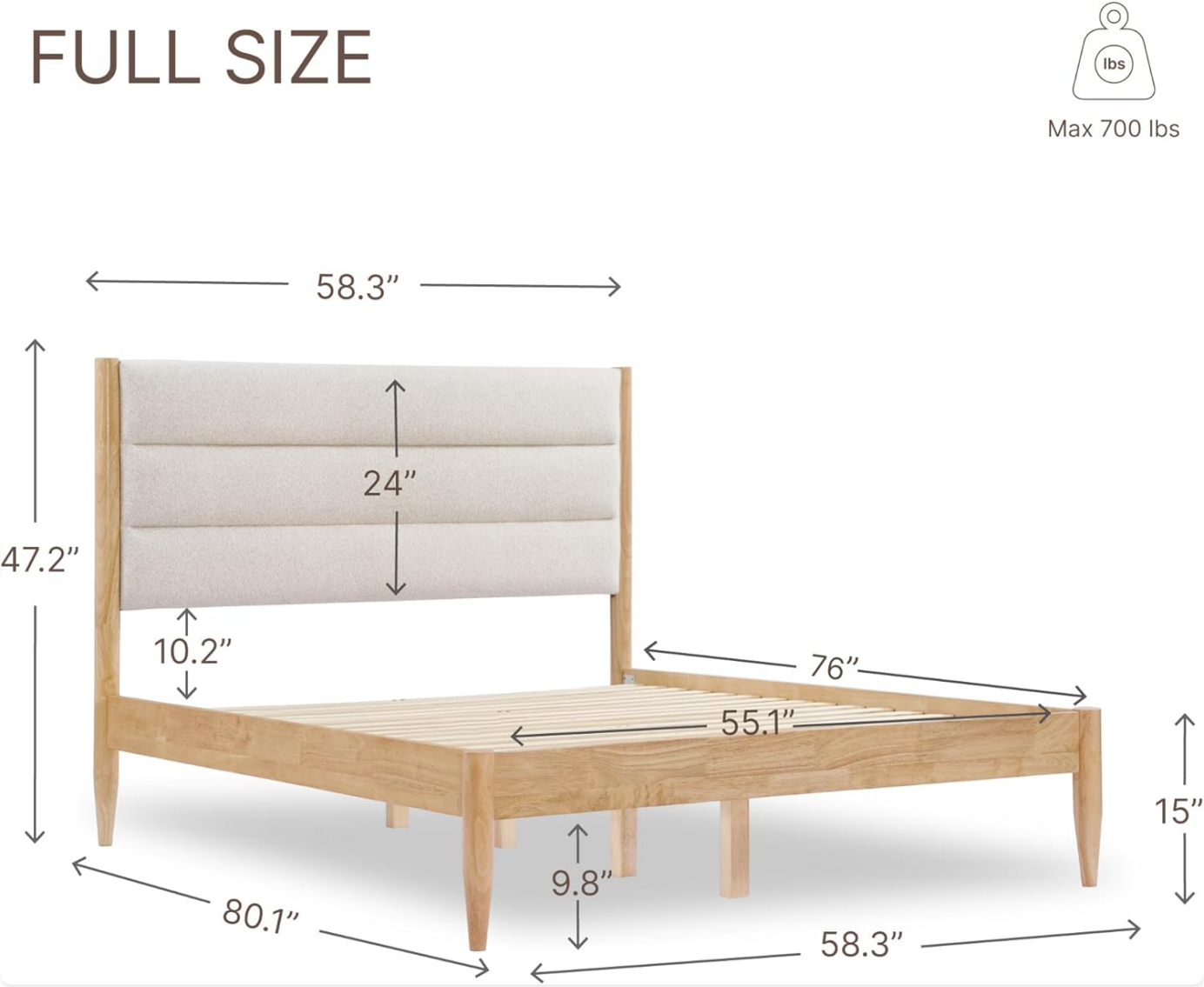
Figure 7.1: Detailed dimensions for the Full Size KISLOT Bed Frame.
