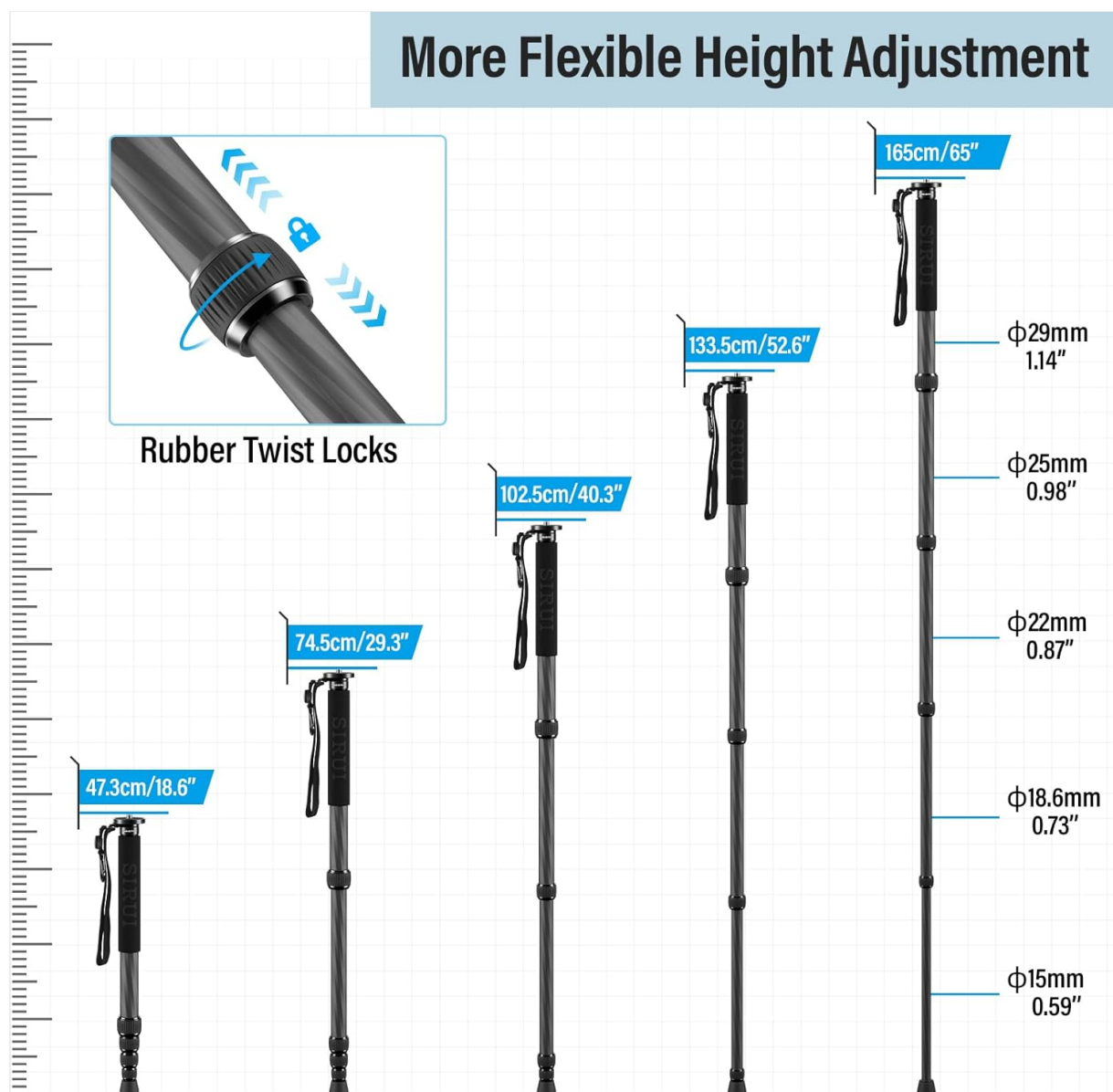
Image: Twist lock mechanism and height adjustment examples.
