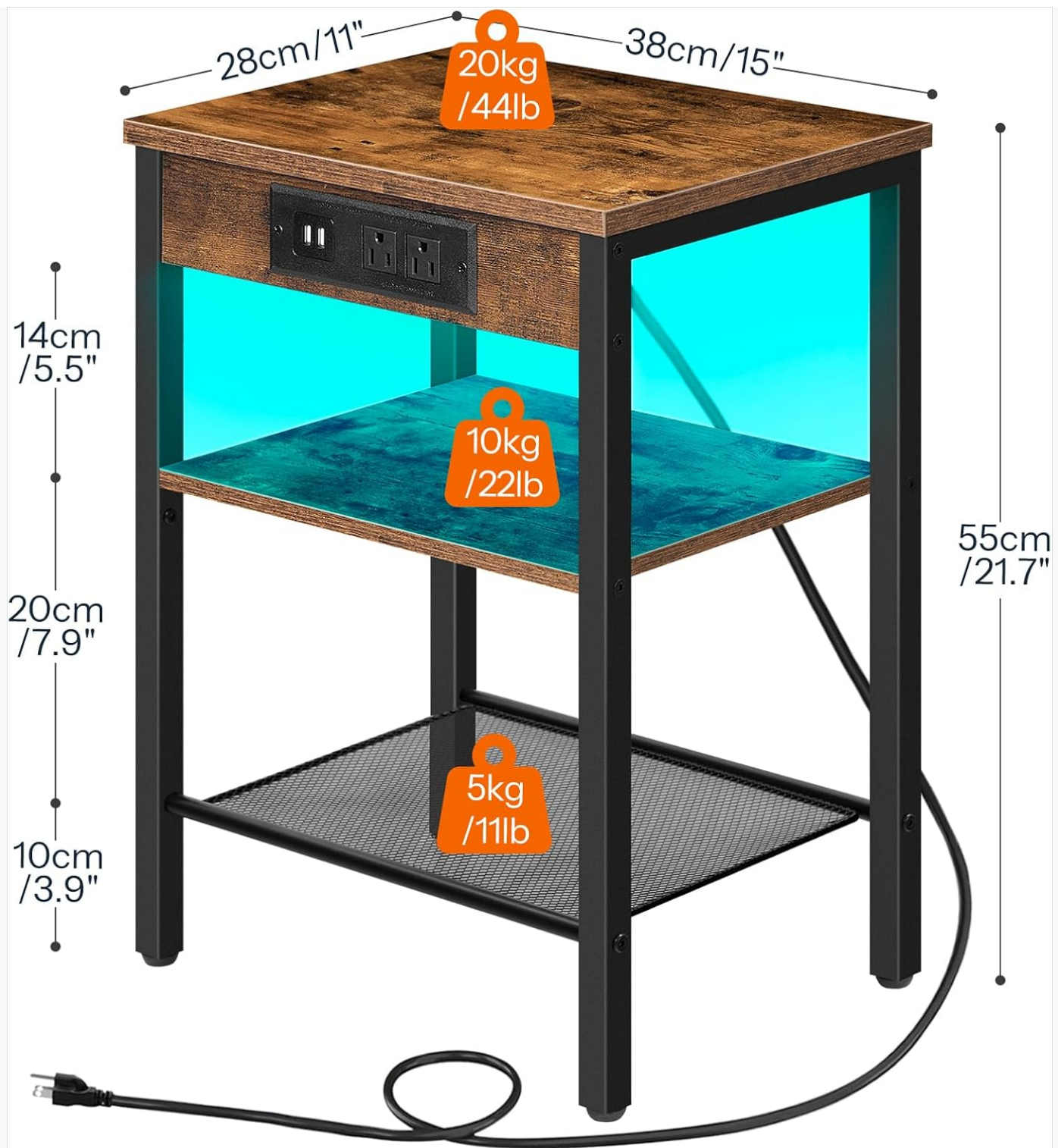
Image: Diagram illustrating the dimensions and weight capacities of the HOOBRO LED Nightstand, showing measurements for height, width, and shelf load limits.
