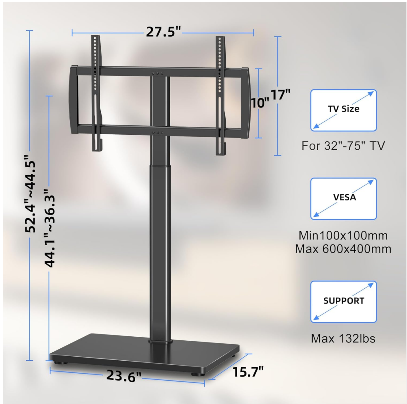
Figure 4.1: Product Dimensions and Compatibility. This diagram illustrates the overall dimensions of the stand, its VESA compatibility (Min 100x100mm, Max 600x400mm), and maximum supported TV weight (132 lbs) for TVs between 32 and 75 inches.
