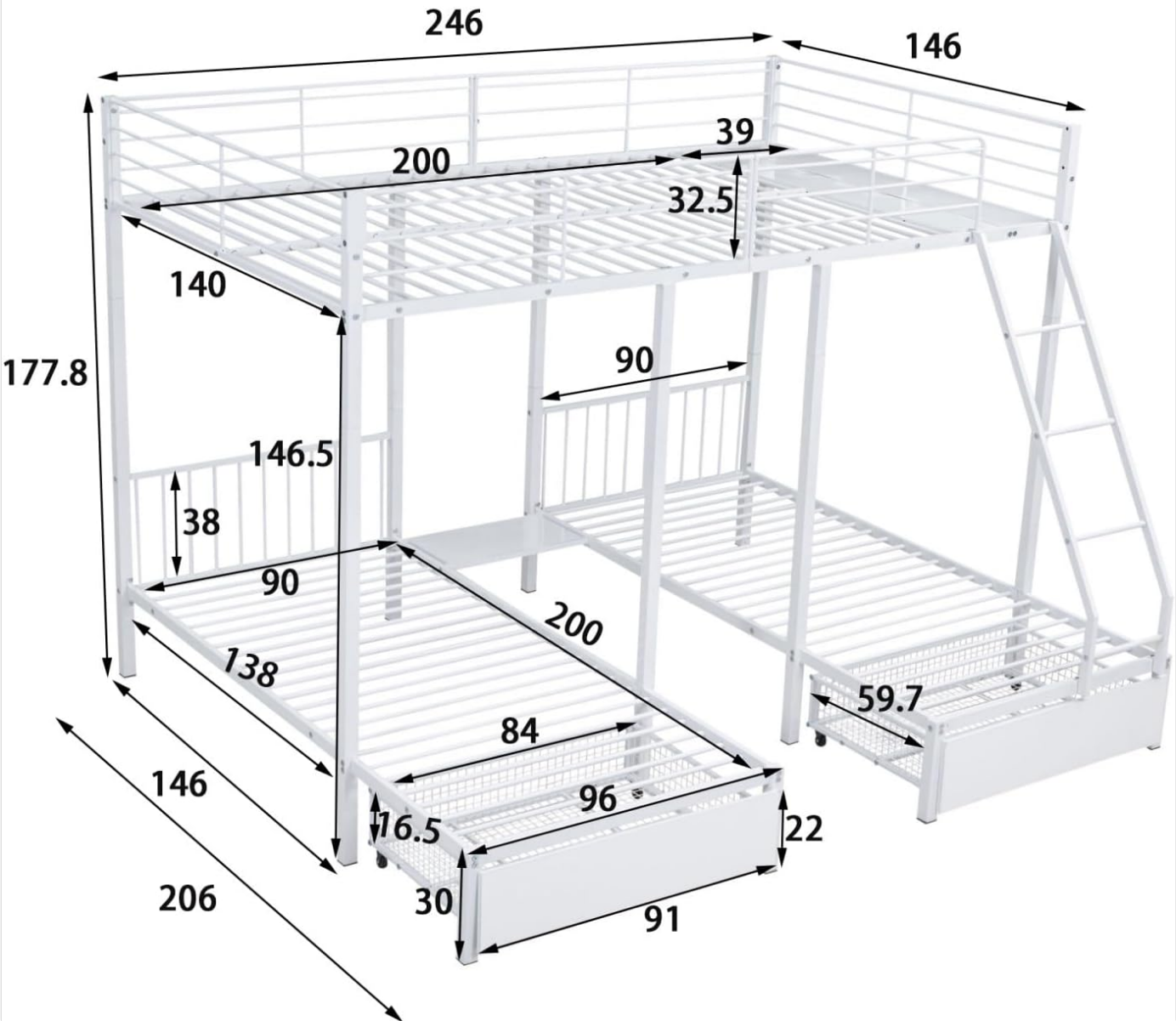
Image 4.1: Dimensional drawing of the KOMHTOM Triple Bunk Bed, showing all key measurements in centimeters.
