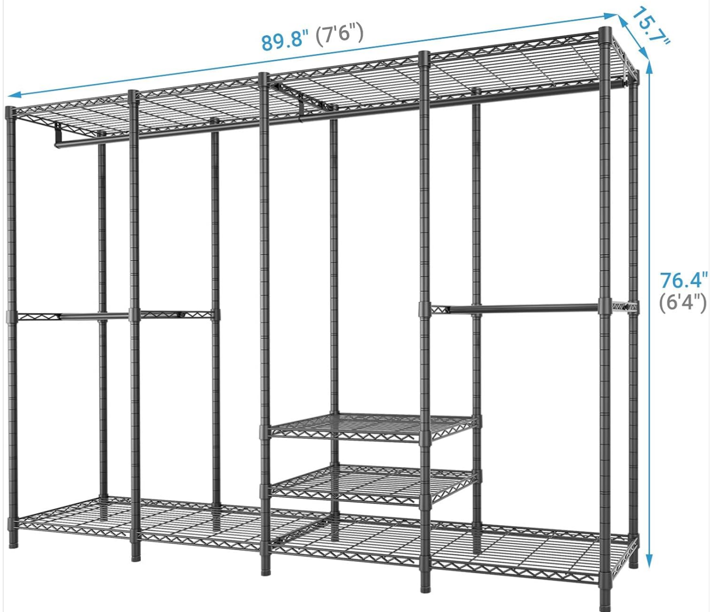
Image 8.1: Product dimensions and weight capacity diagram.
