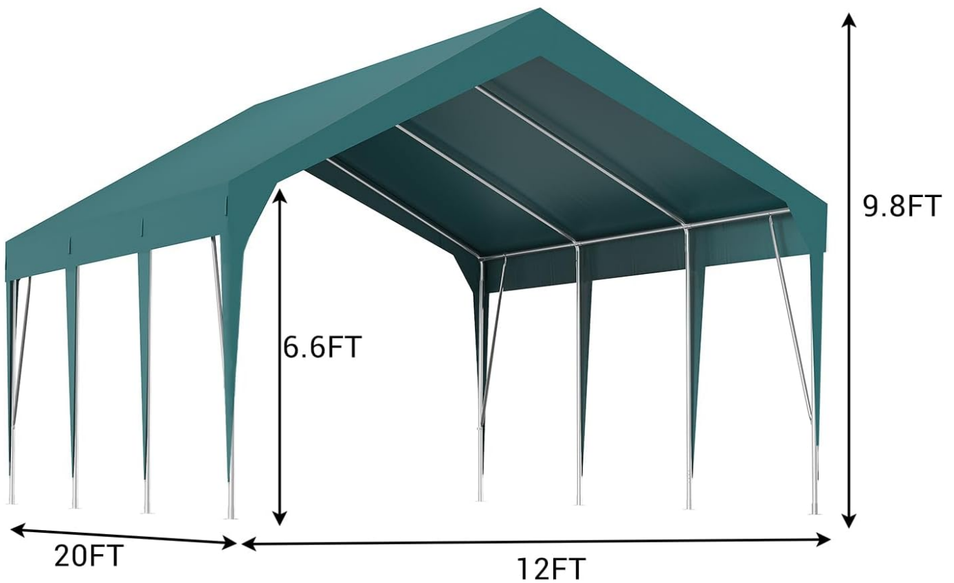
Image 3: Product size diagram illustrating the dimensions of the carport.
