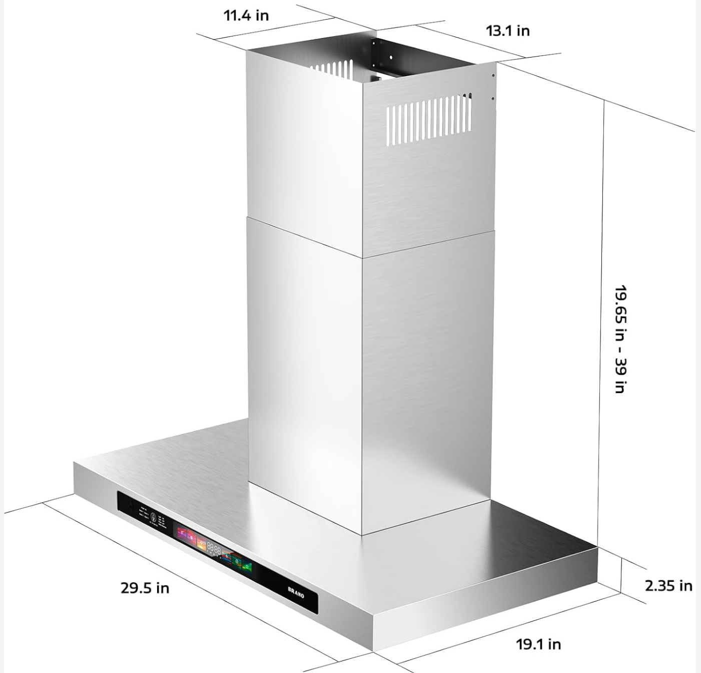
Figure 4.1: Product dimensions for installation planning.
