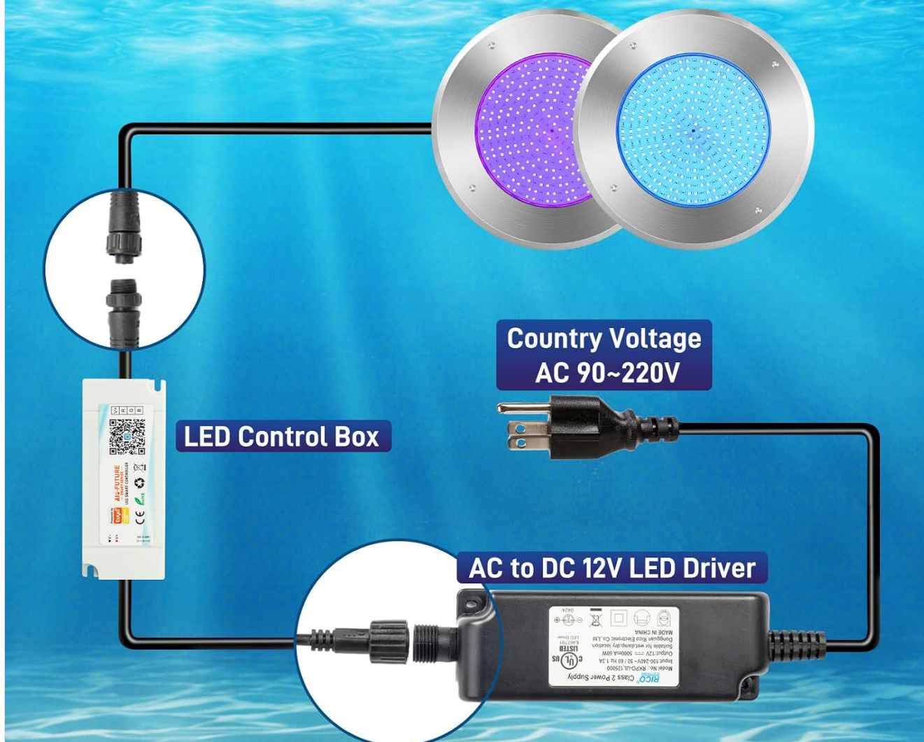
Figure 4.1: Connection diagram for the VINGLI pool light system, illustrating the flow from the AC power source to the LED driver, then to the LED control box, and finally to the pool light.
