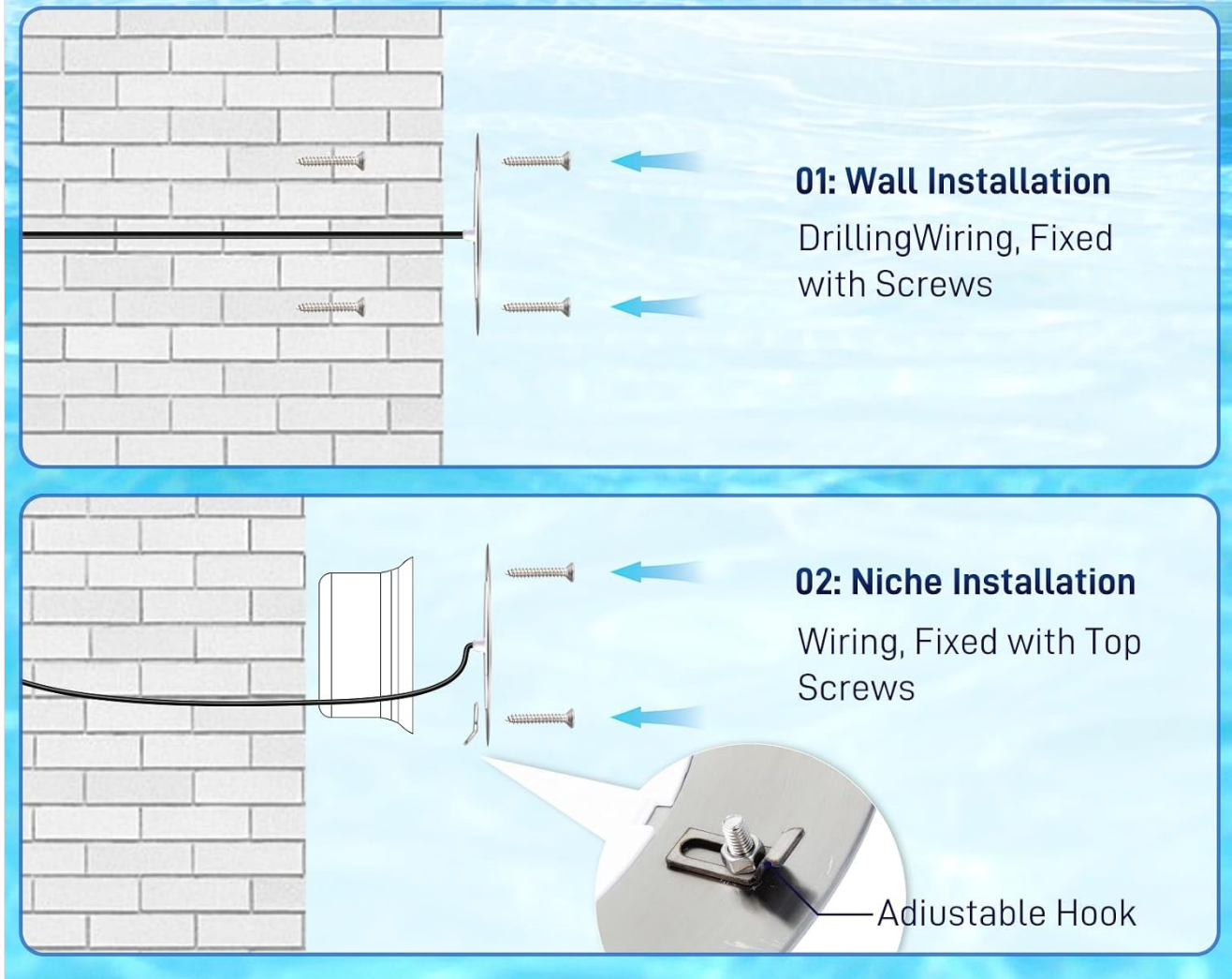
Figure 4.3: Visual guide for two installation methods: Wall Installation (drilling, wiring, fixed with screws) and Niche Installation (wiring, fixed with top screws, utilizing an adjustable hook).
