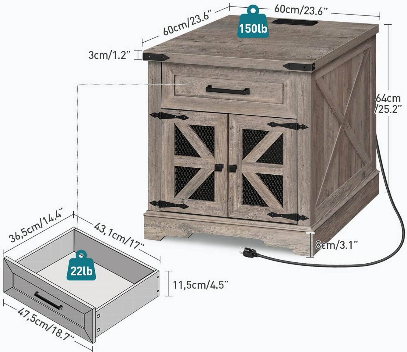
Image 2.1: Detailed diagram illustrating the product dimensions and weight capacities.
